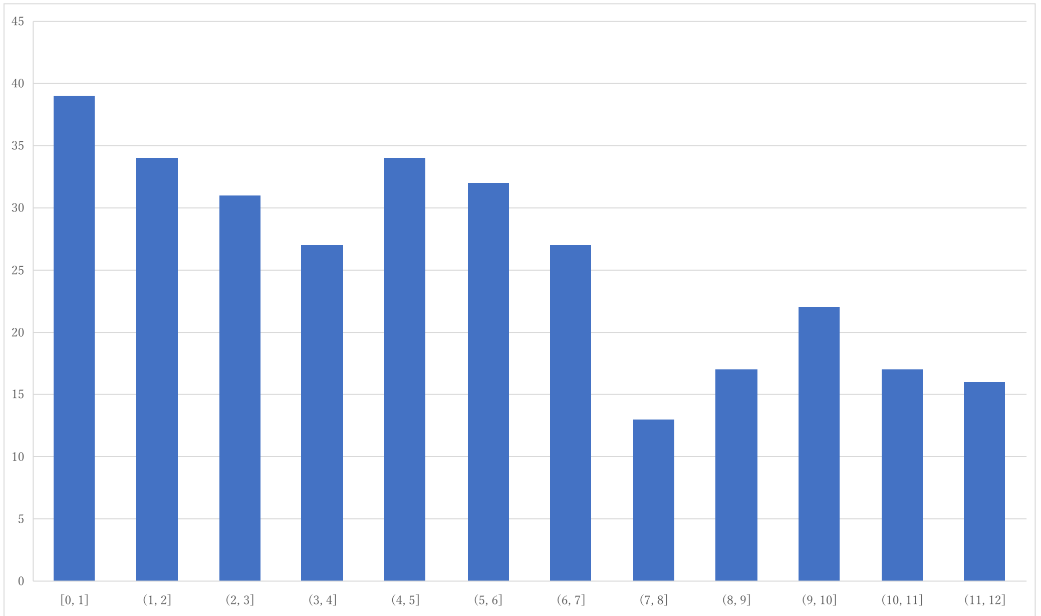
Histogram of P5
