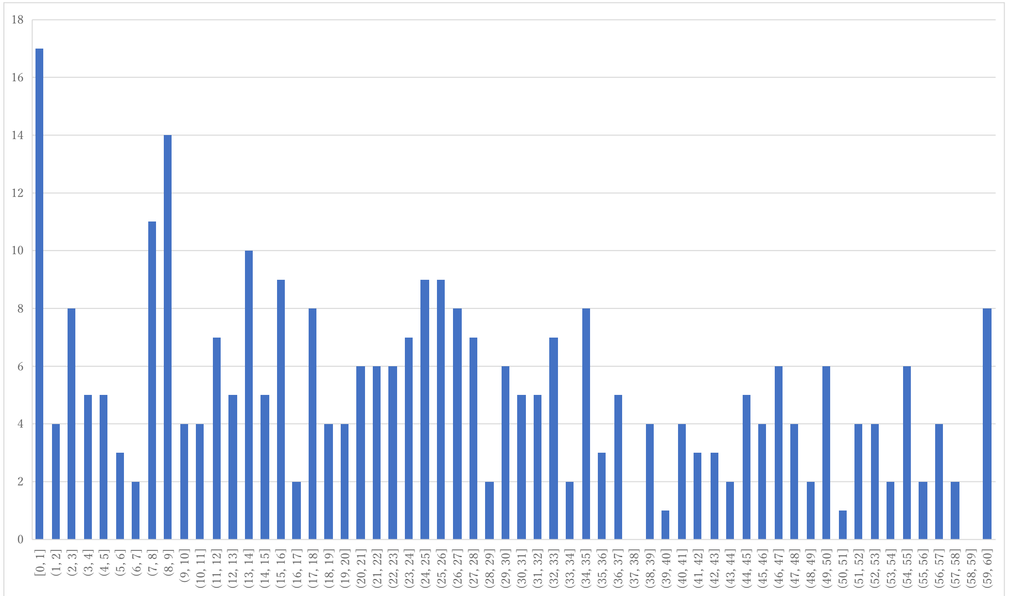
Histogram of P5 (raw point)
