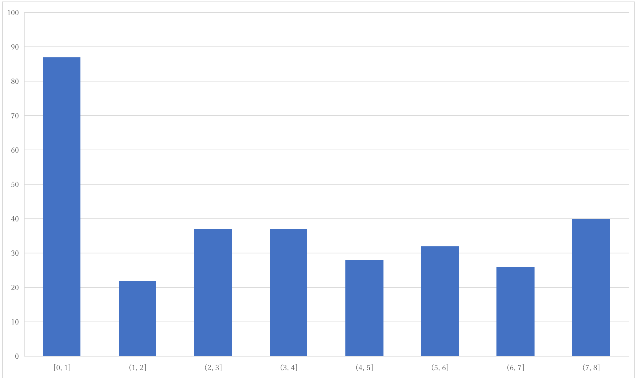
Histogram of P3
