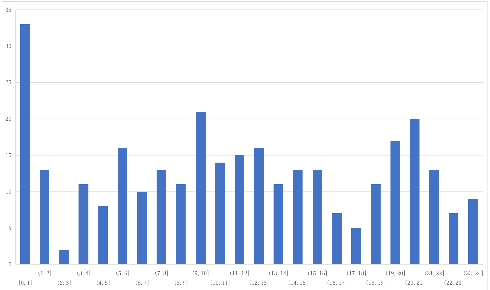
Histogram of P1 (raw point)
