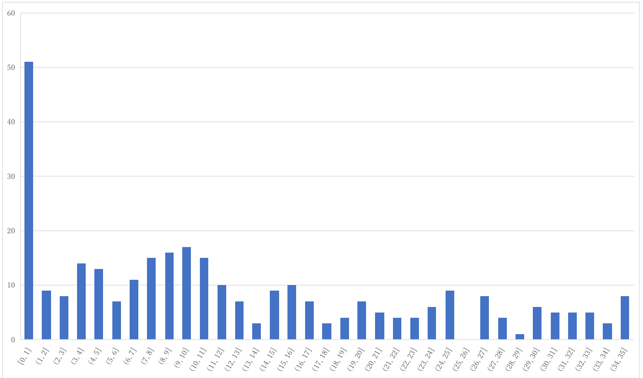
Histogram of P2 (raw point)
