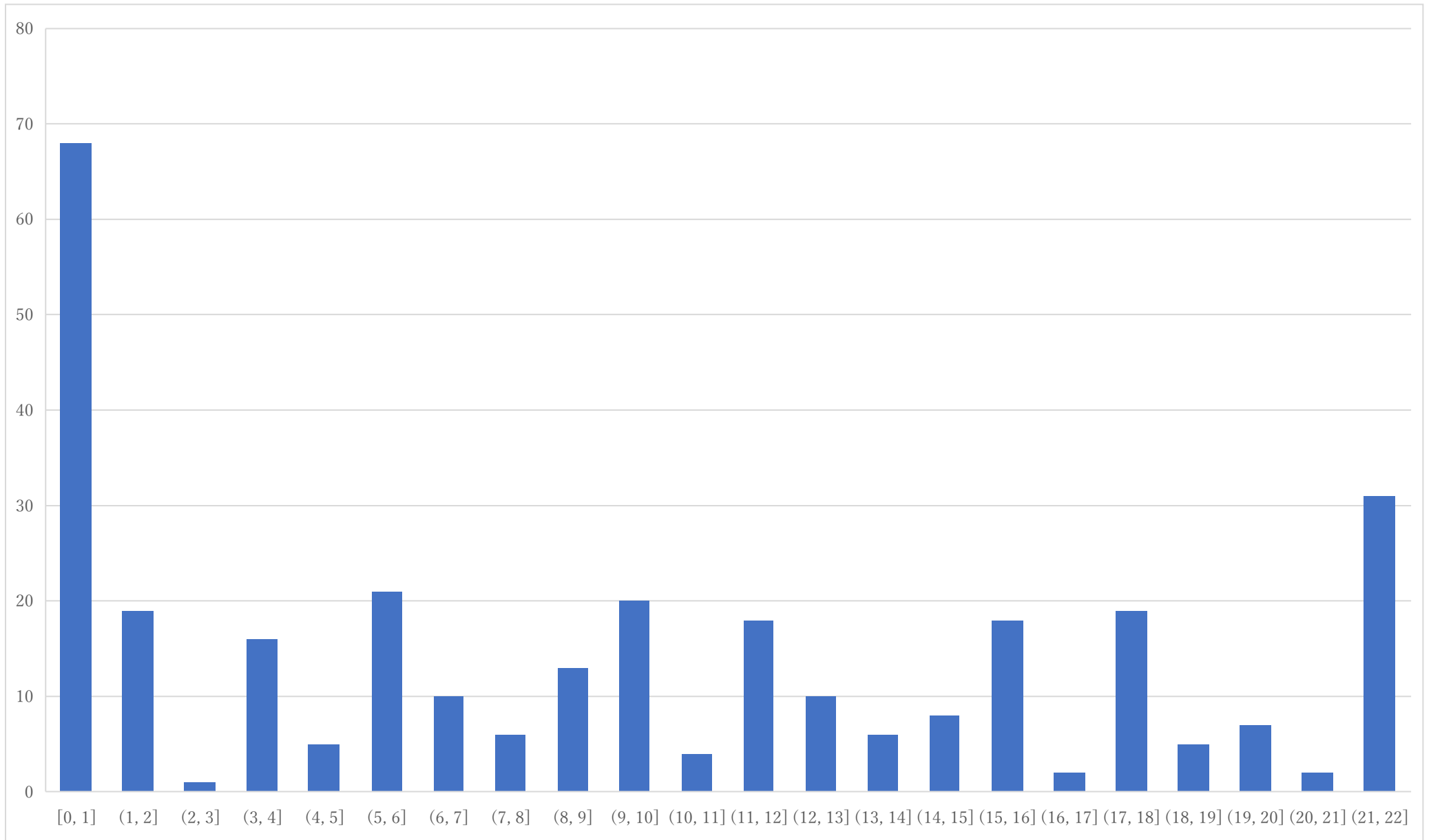
Histogram of P3 (raw point)
