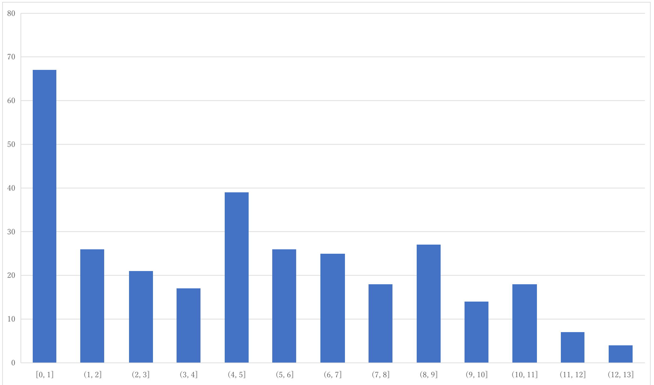
Histogram of P6
