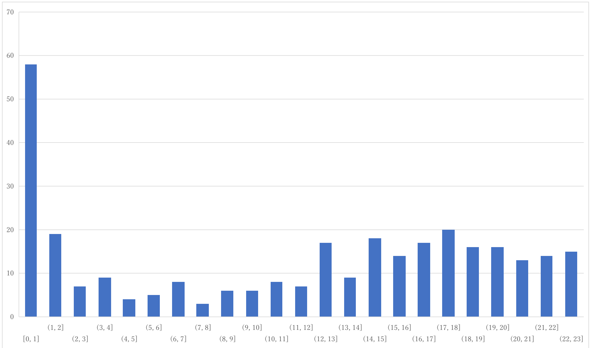
Histogram of P9 (raw point)
