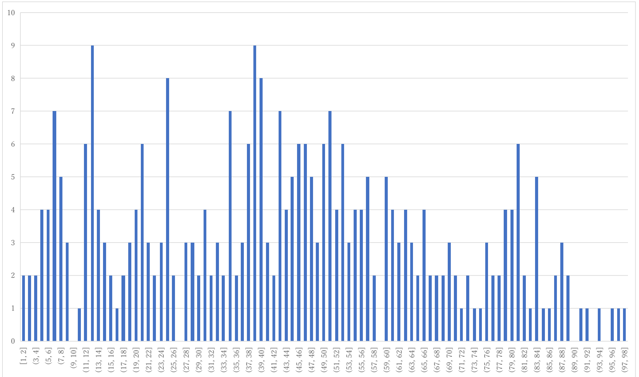
Histogram of Total Scores
