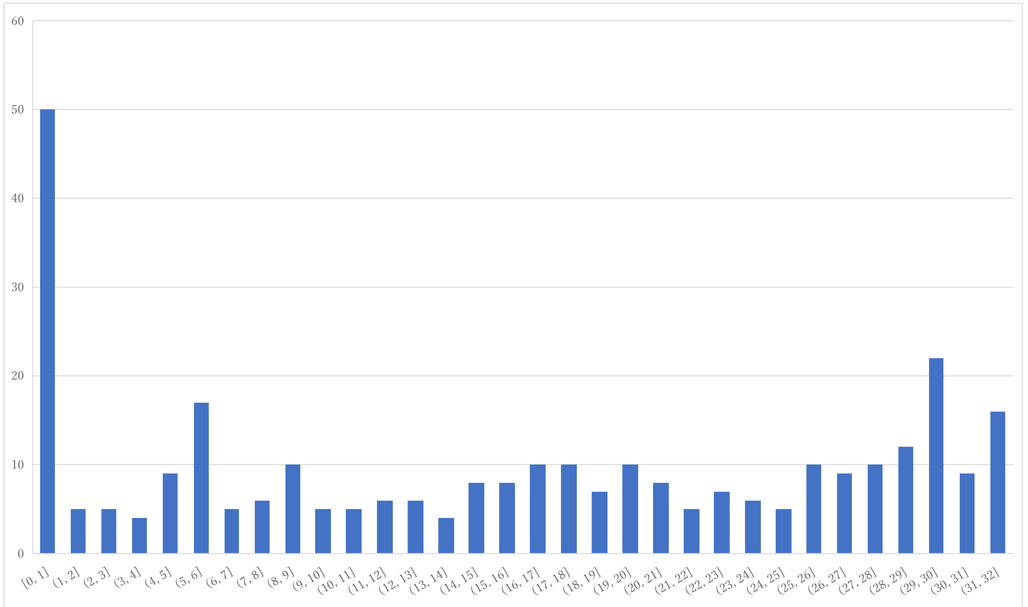
Histogram of P4 (raw point)
