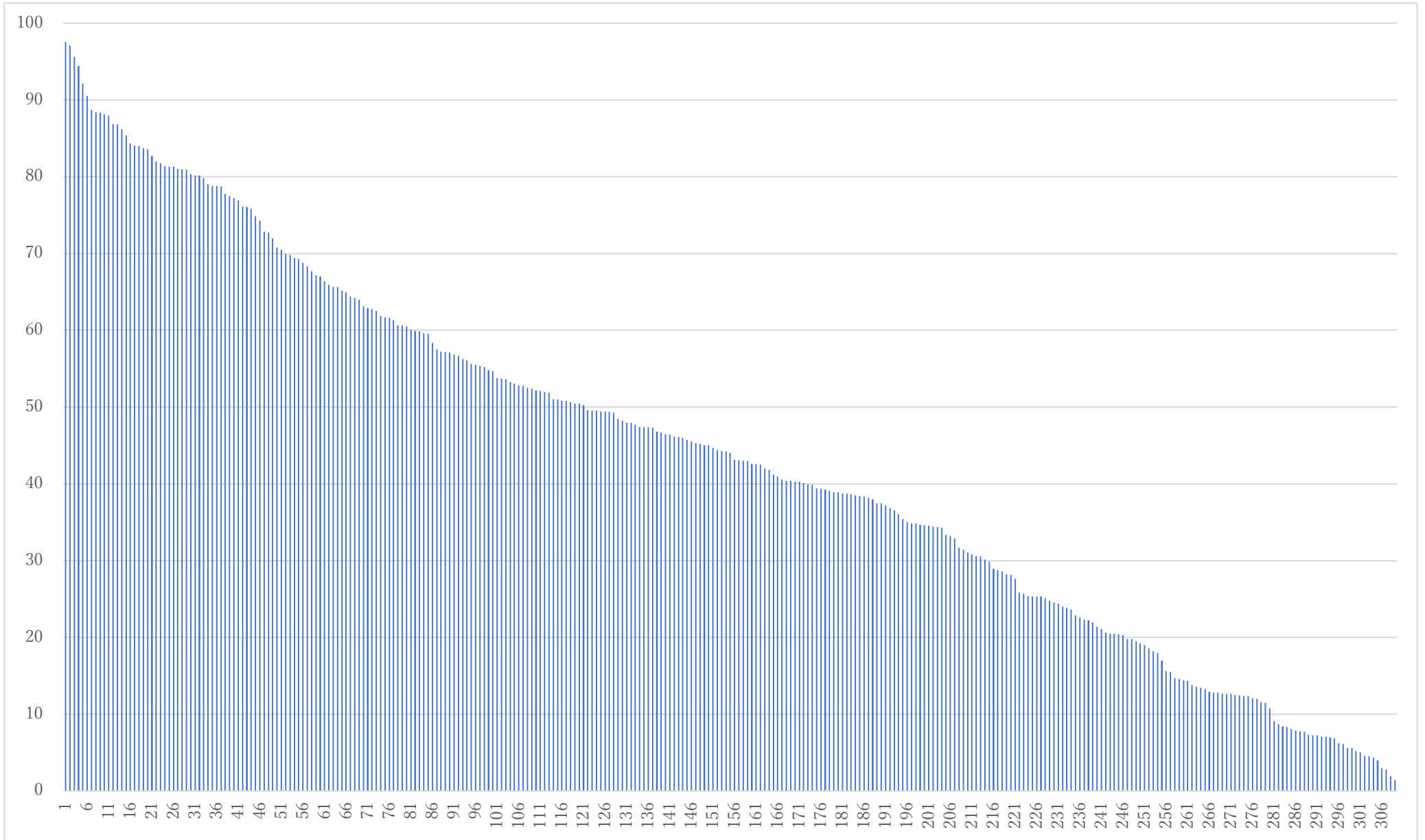
Distribution of Total Scores
