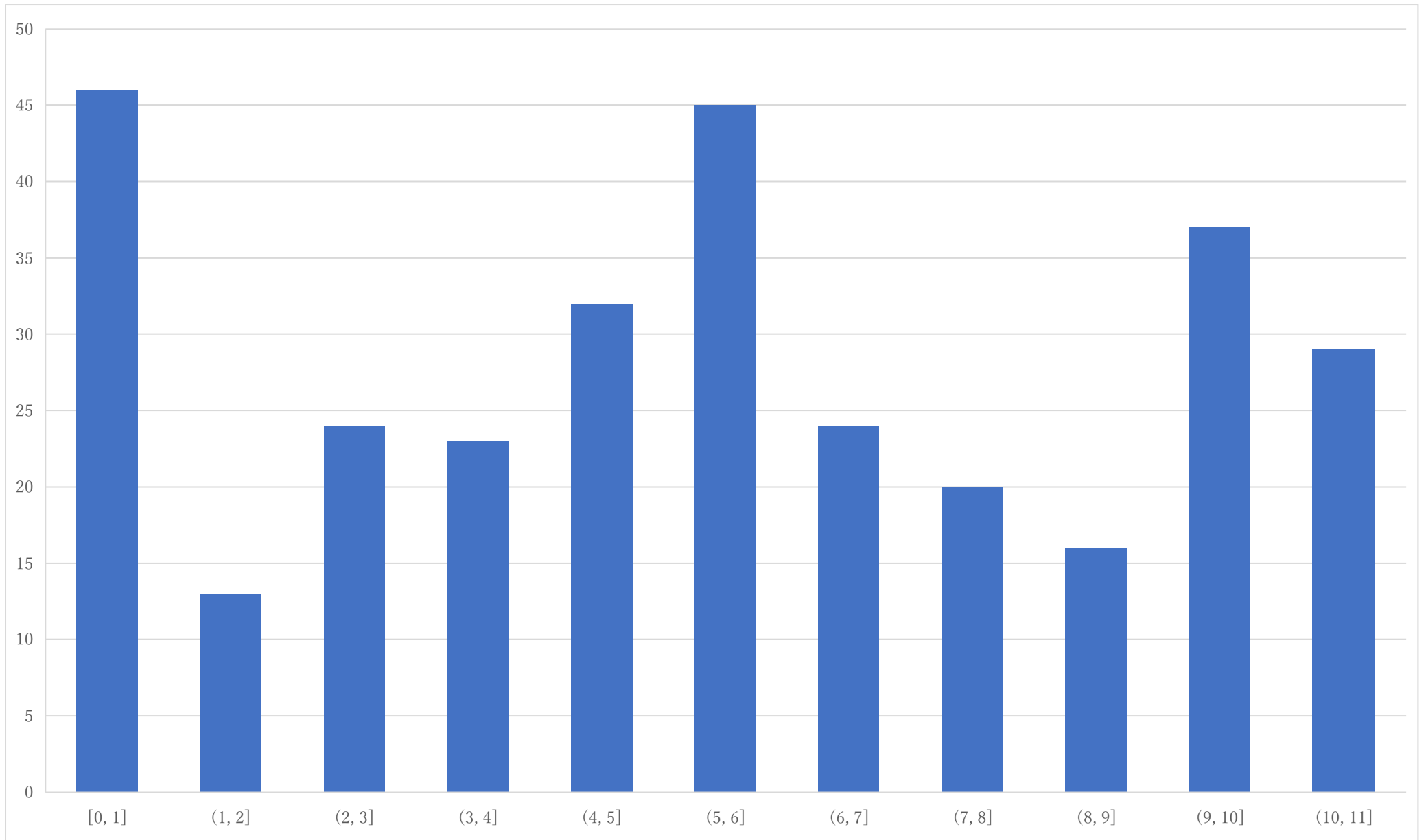
Histogram of P1
