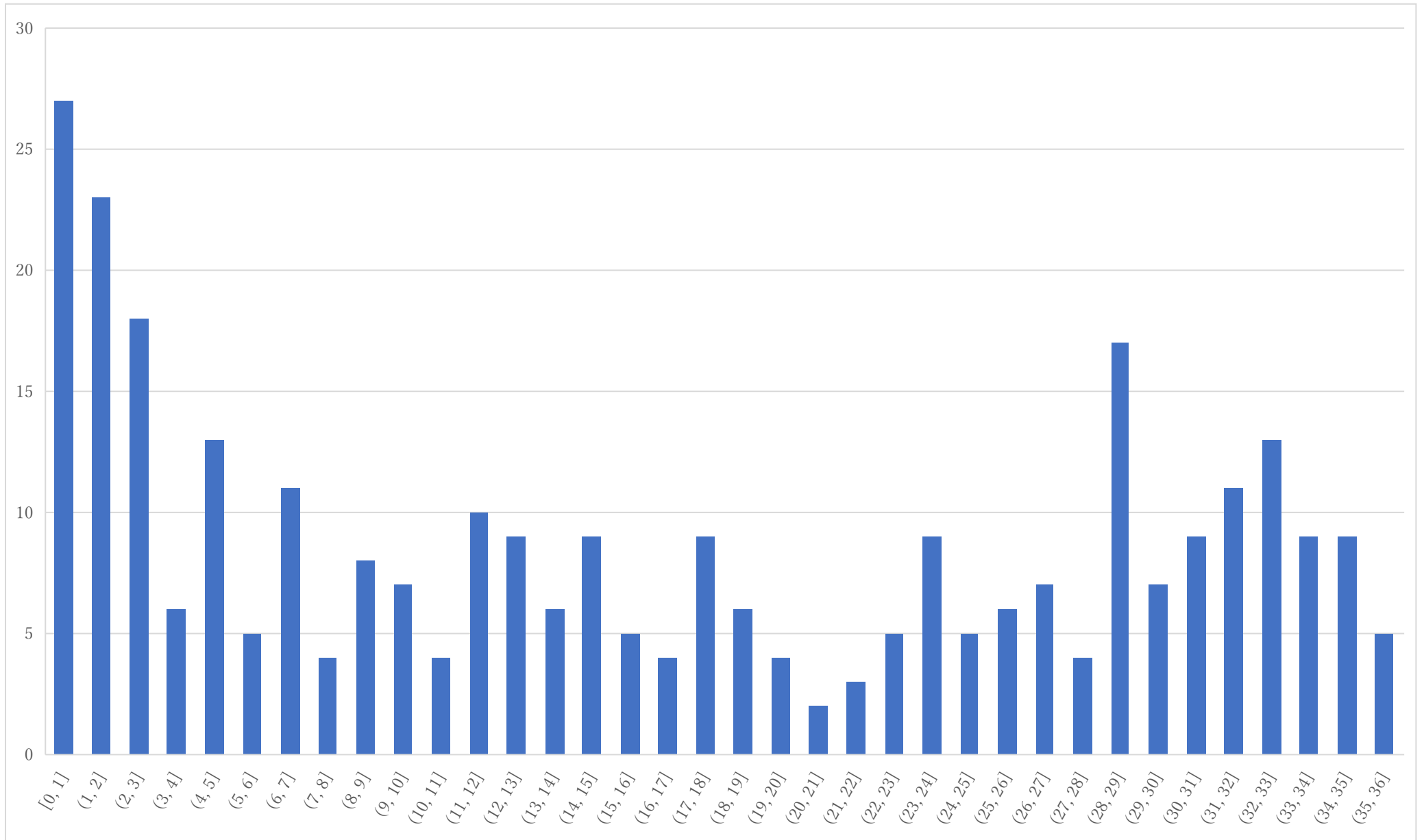
Histogram of P7 (raw point)
