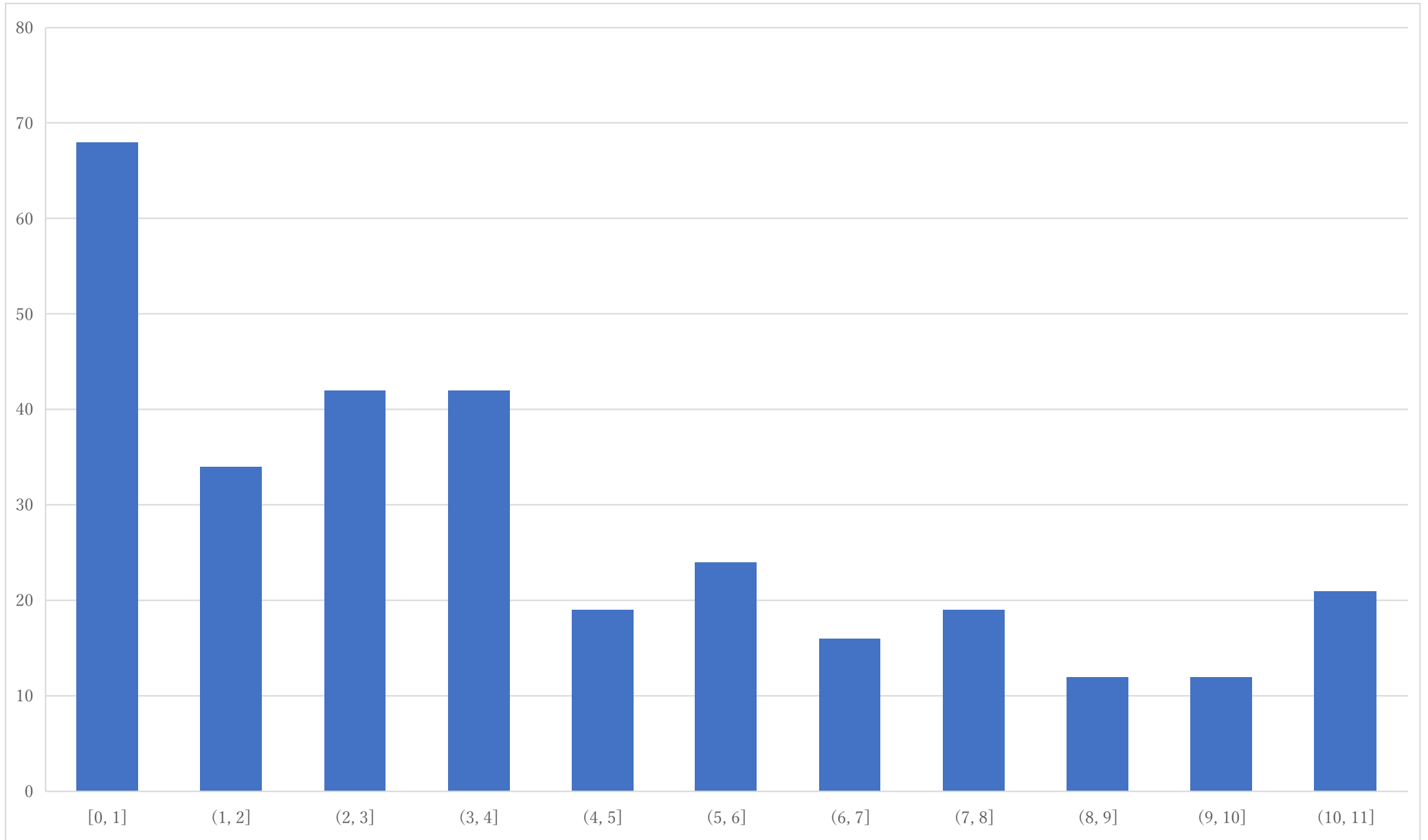
Histogram of P2
