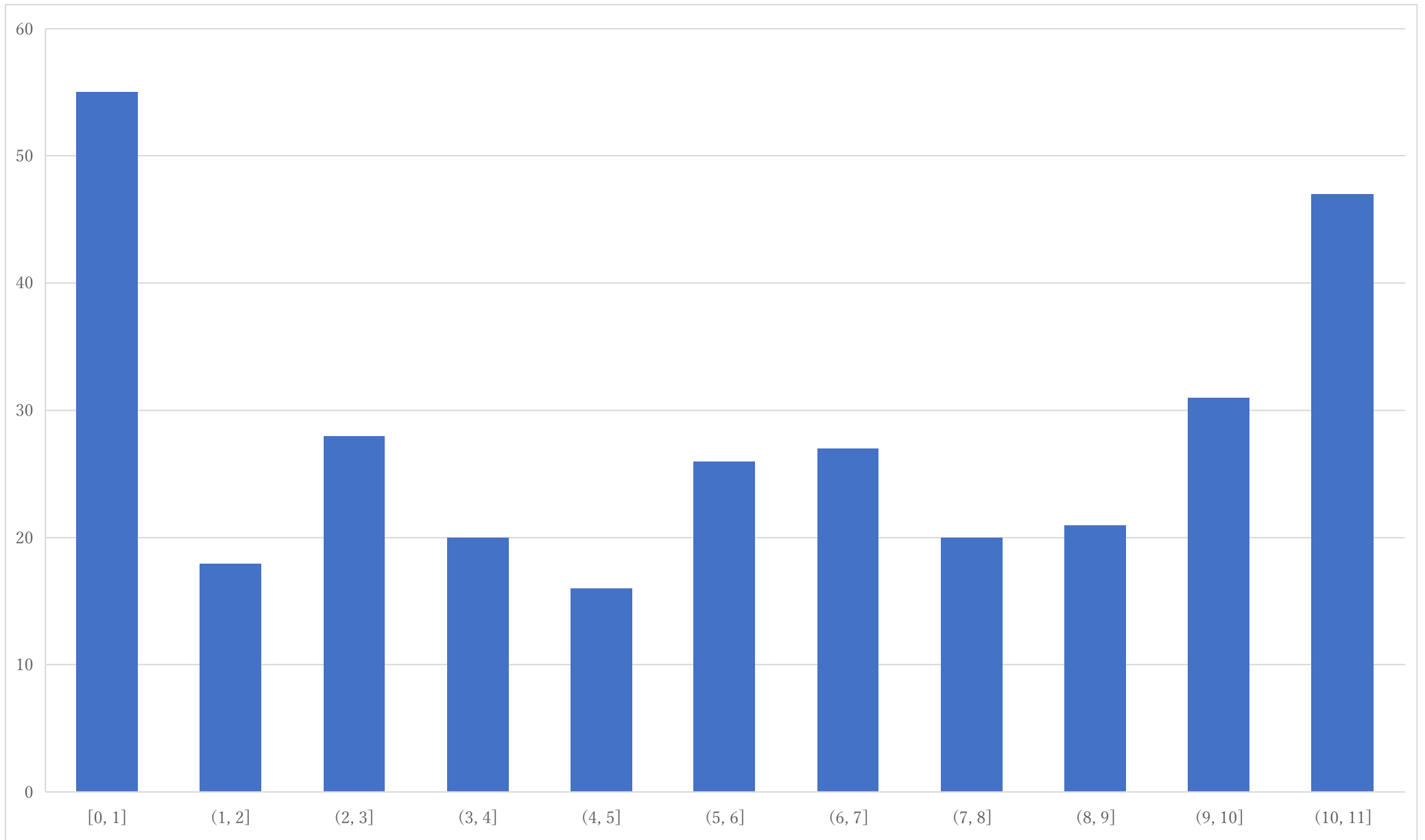
Histogram of P4
