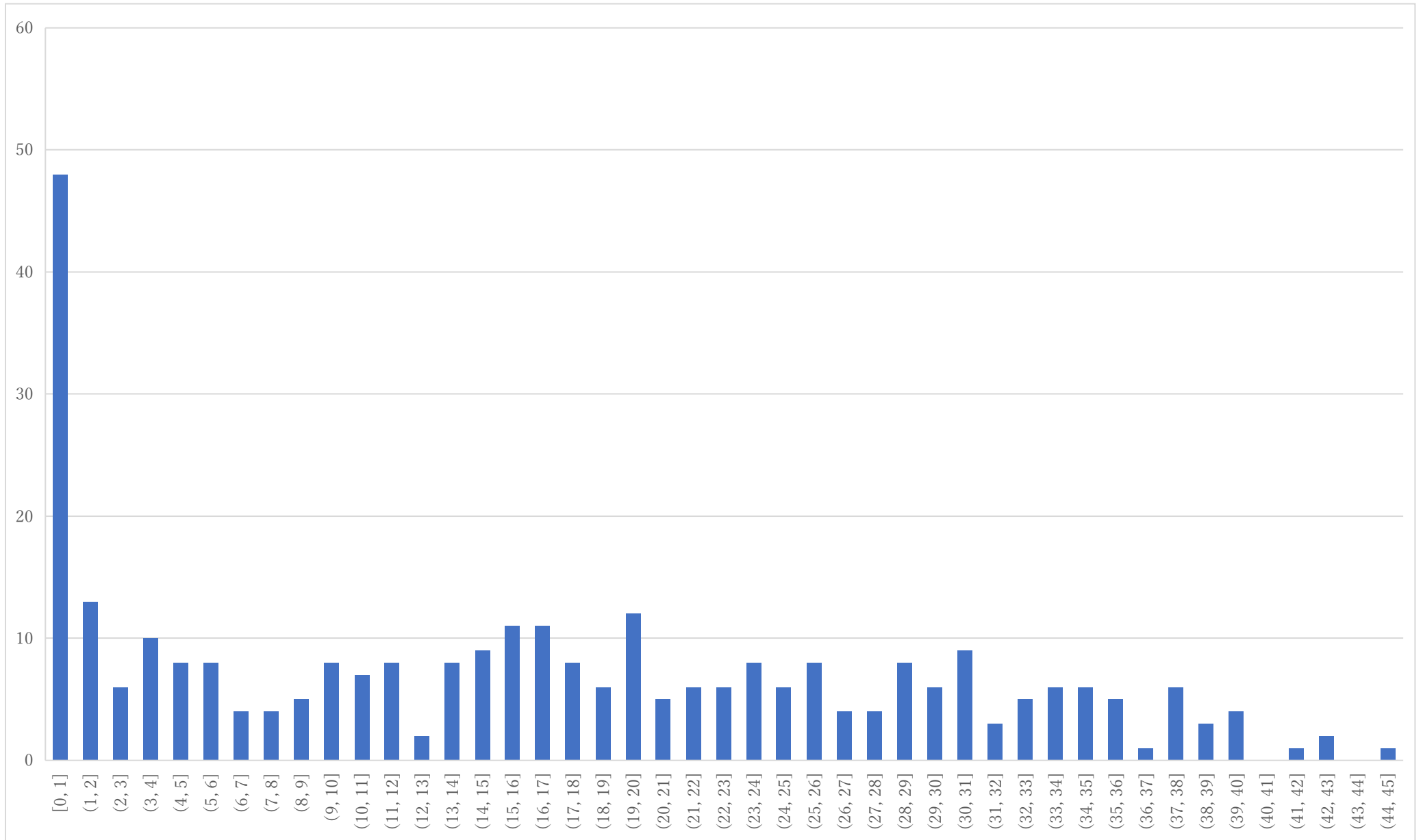
Histogram of P6 (raw point)
