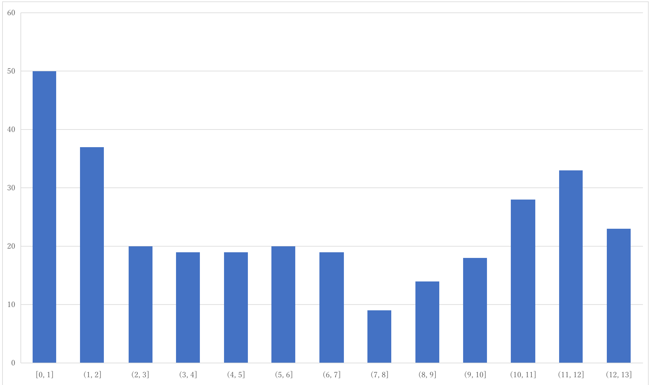
Histogram of P7
