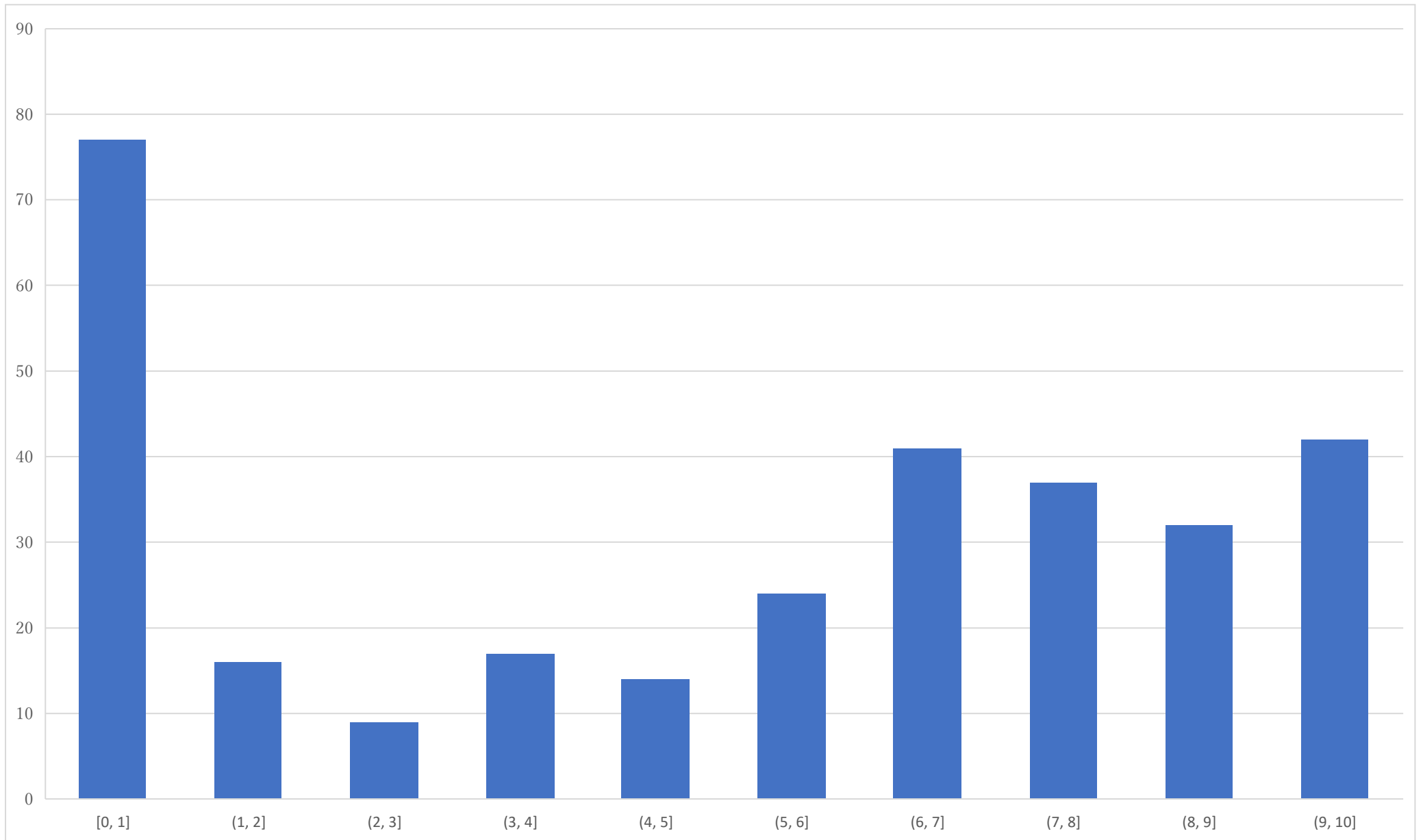
Histogram of P9
