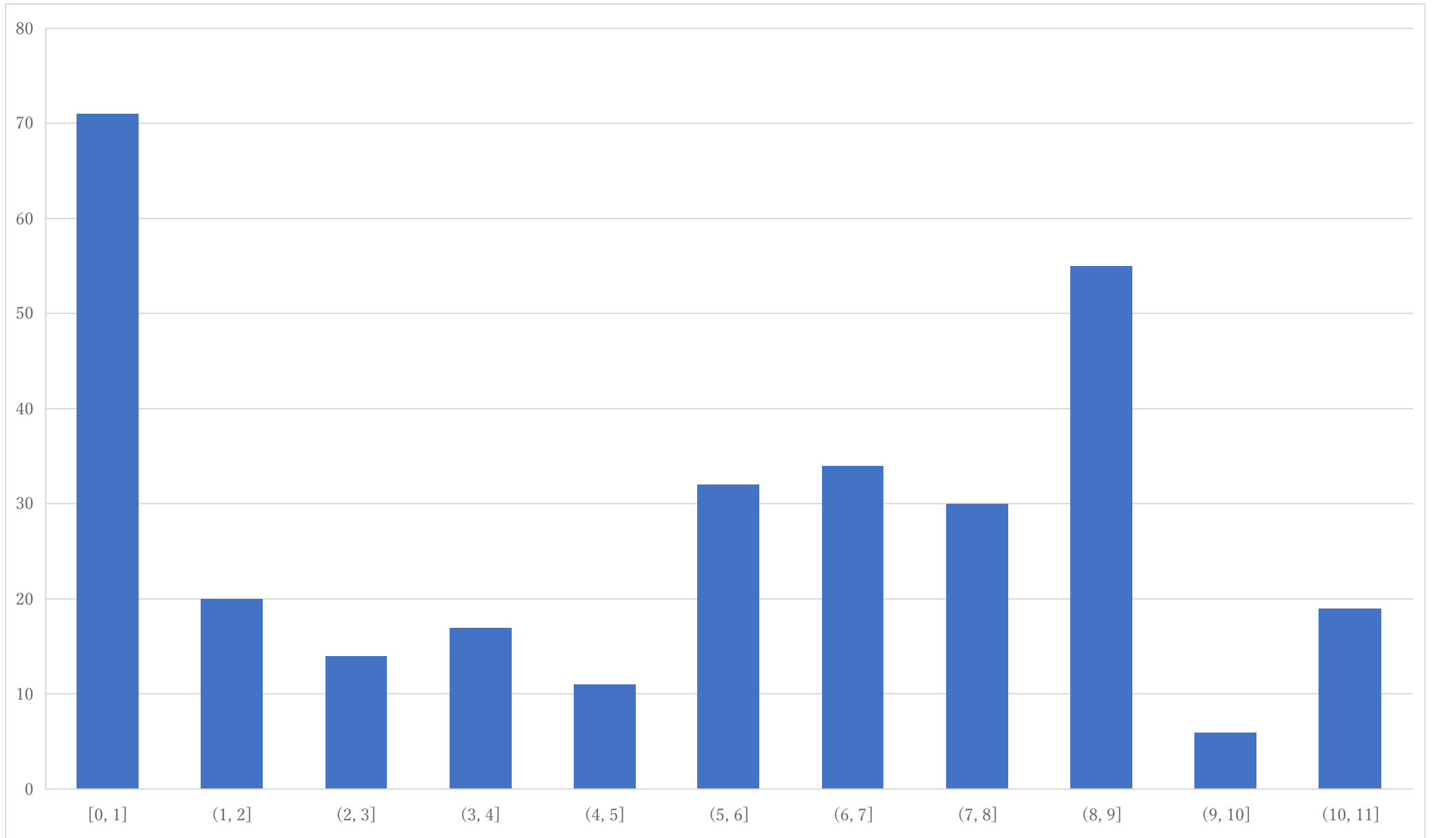
Histogram of P8
