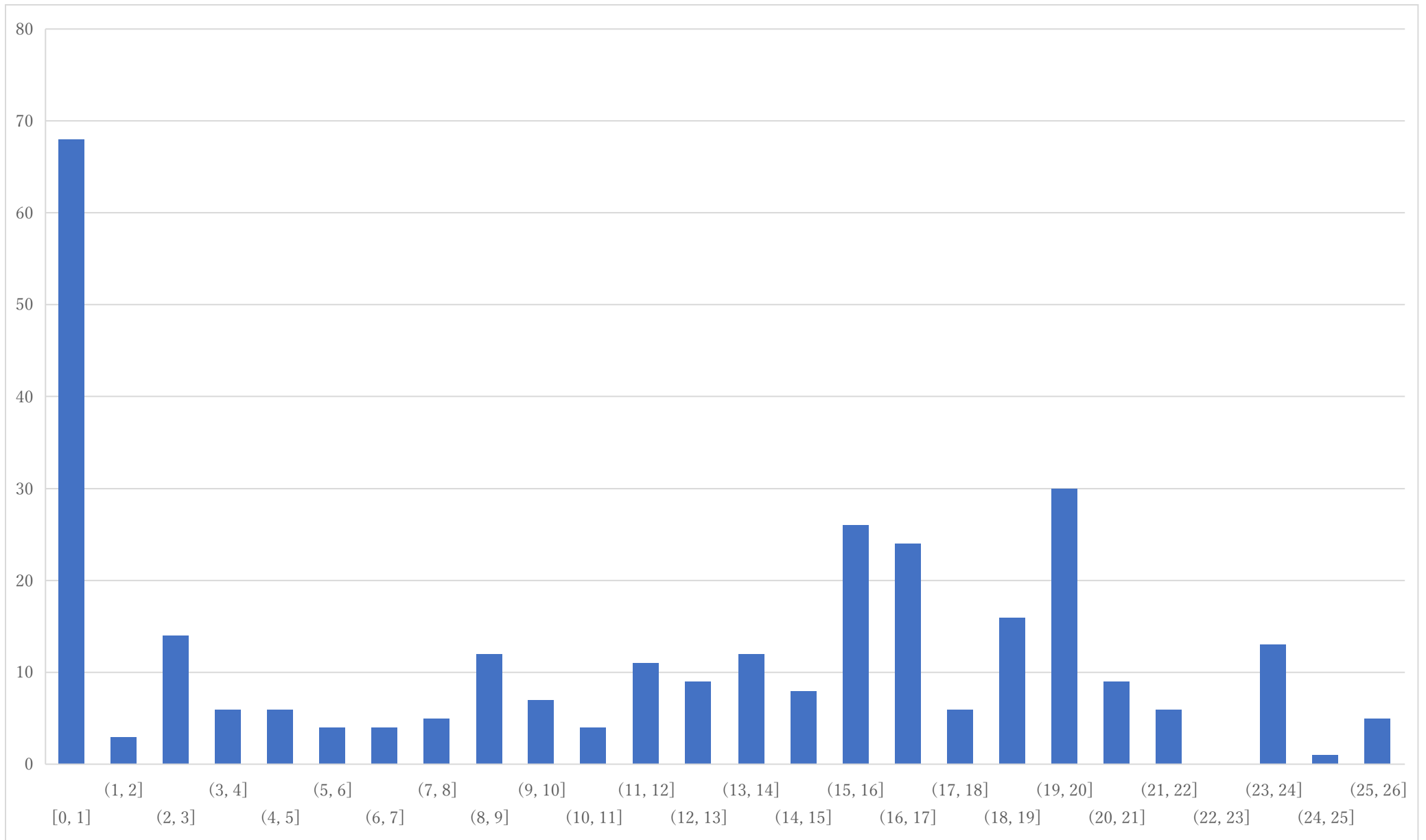
Histogram of P8 (raw point)
